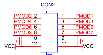
HEADER-DIP2x6-254-FEMALE HEADER-DIP2x6-254-FEMALE-TOP
