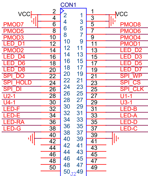
HEADER-DIP2x25-254-Male HEADER-DIP2x25-254-Male-BOT
